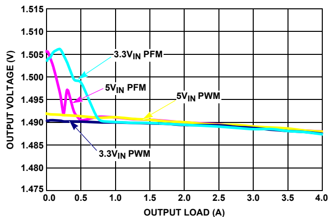
FIGURE 9. V OUT REGULATION vs LOAD (1MHz, V OUT = 1.5V)
