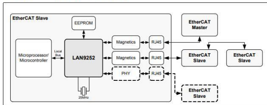
FIGURE 2-1: SYSTEM BLOCK DIAGRAM
