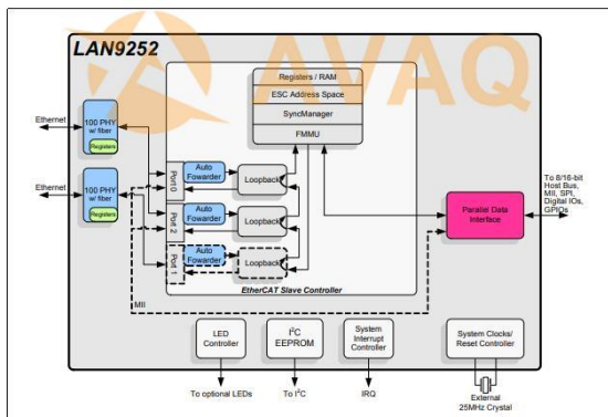
FIGURE 2-2: INTERNAL BLOCK DIAGRAM
