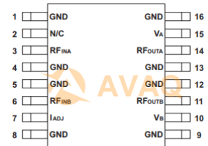
Figure 2: Pin Out
