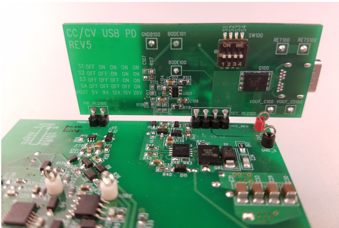
Figure 3. Bottom View of the Daughter Card
